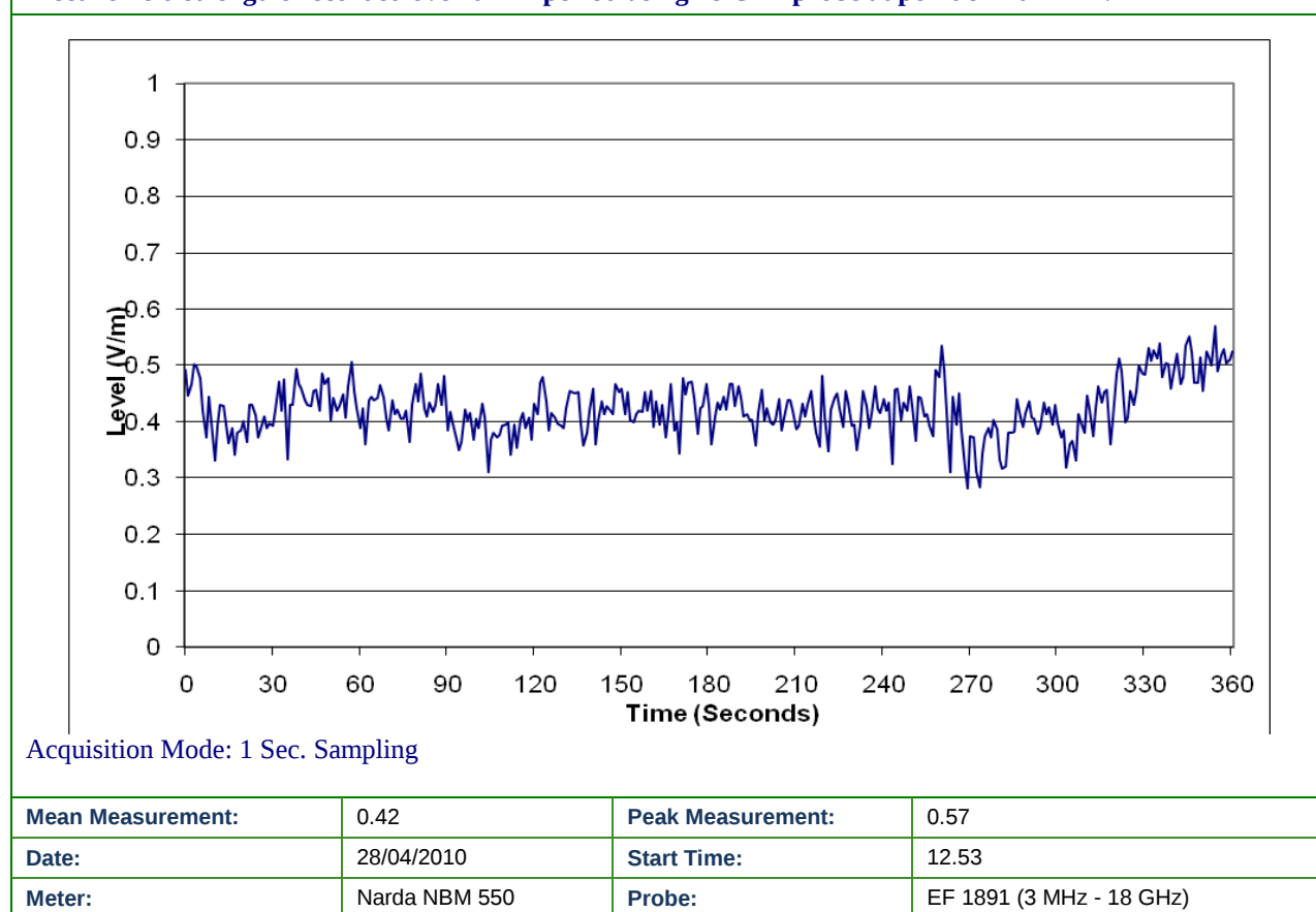
Electric field strengths recorded over 6 min period using 18 GHz probe at point of max NIR:
